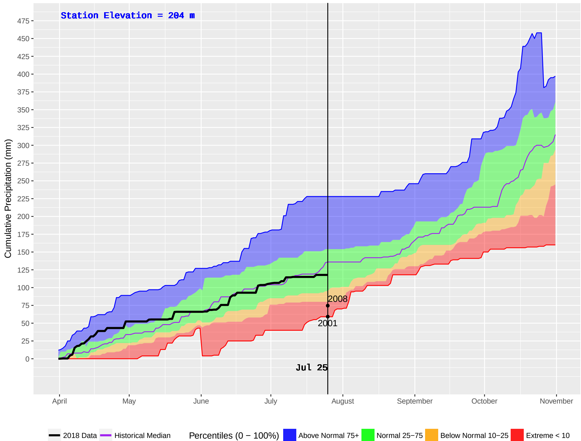
PEMBERTON BASE (301) : Historical (2001–2016) and Current (2018) Noon Cumulative Precipitation
