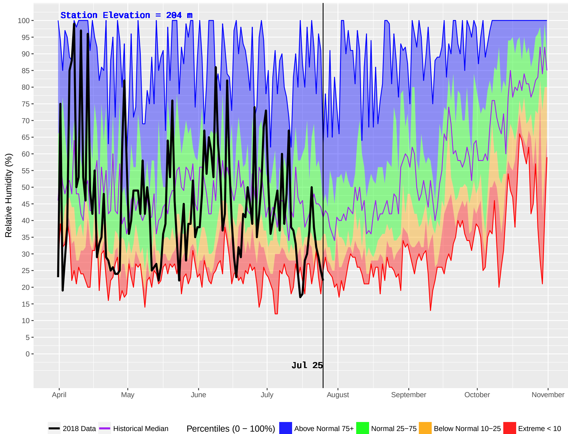
PEMBERTON BASE (301) : Historical (2001–2016) and Current (2018) Noon Relative Humidity
